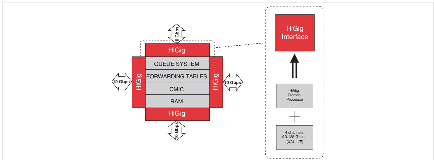
Nonblocking 8-Port Gigabit Ethernet Switch
