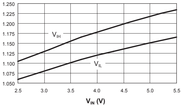
LDO SHDN V_{IH} and V_{IL} vs. V_{IN}
