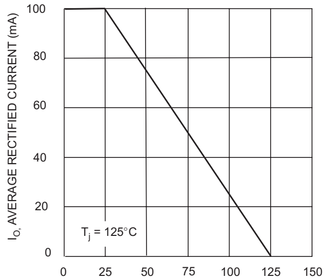
T_A , AMBIENT TEMPERATURE (°C) Fig. 2 Forward Current Derating Curve (Per Element)
