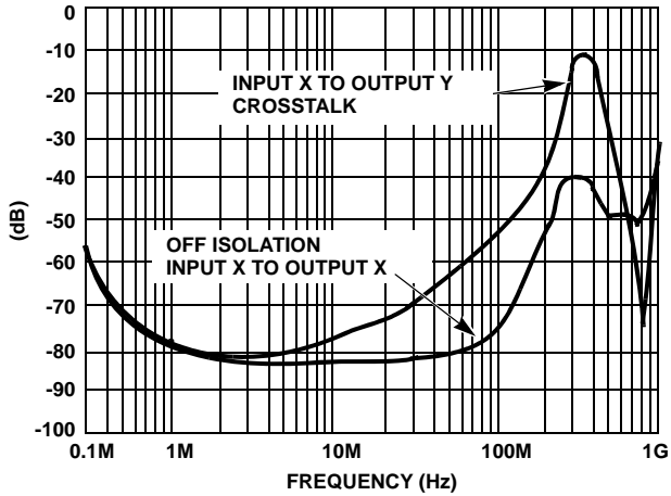
FIGURE 13. MUX1: CROSSTALK AND OFF ISOLATION
