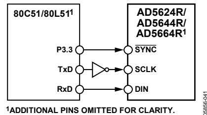
Figure 59. 80C51/80L51 Interface to AD5624R/AD5644R/AD5664R
