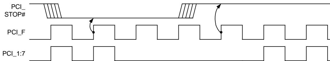
Figure 3: PCI_STOP# Timing
