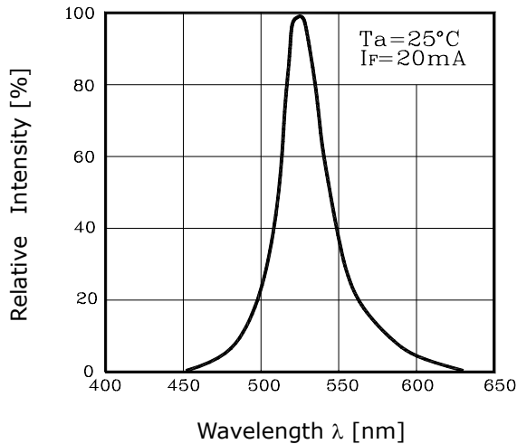
Fig. 4 Spectrum Distribution
