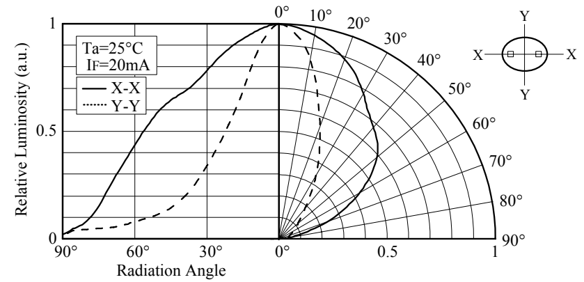
■ Directivity (NSPG546BS)
