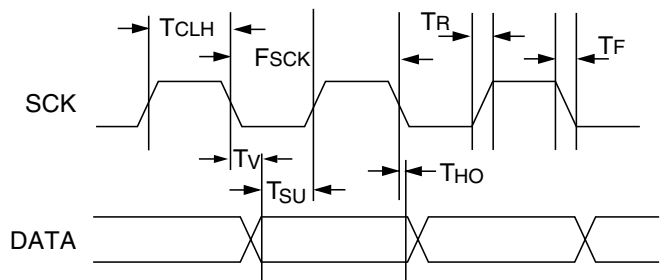
Figure 9 Timing Diagram
