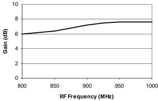
Figure 1. Conversion Gain V_{CC} = 5.0\text{ V} , RF = 940 MHz, IF = 200 MHz
