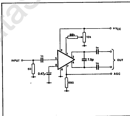
Fig. 3 Test circuit
