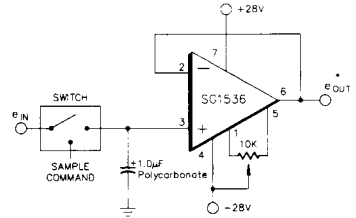
FIGURE 8 - LOW-DRIFT SAMPLE AND HOLD
