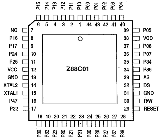
Figure 4. 44-Lead PLCC Package
