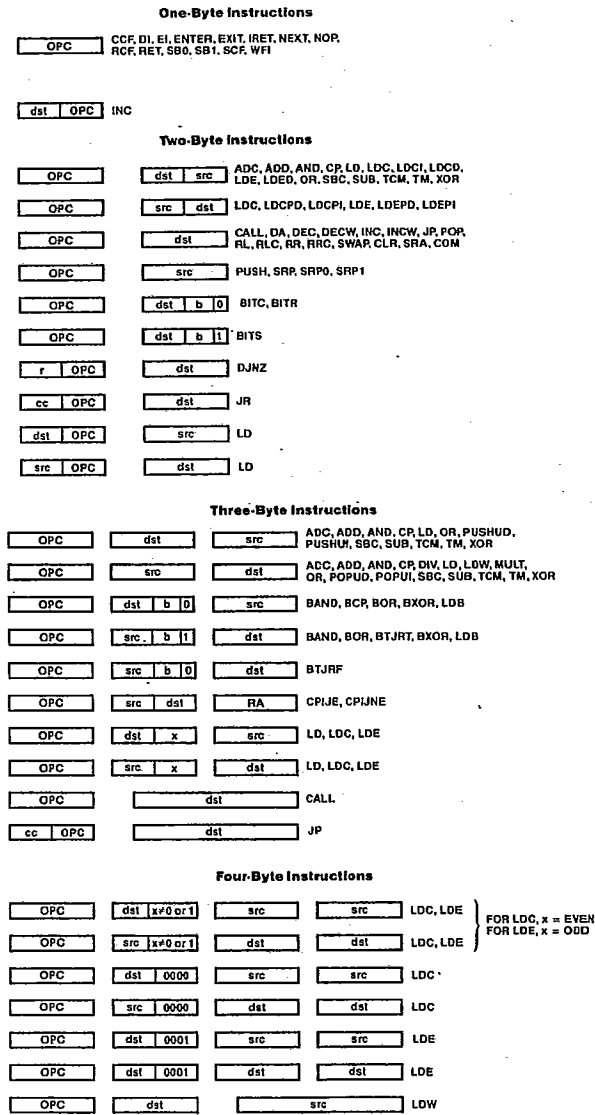
Figure 10. Instruction Formats
