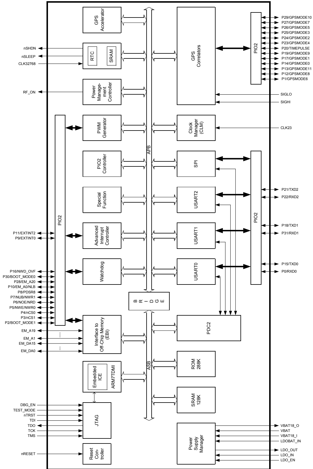
Figure 1-1. Block Diagram
