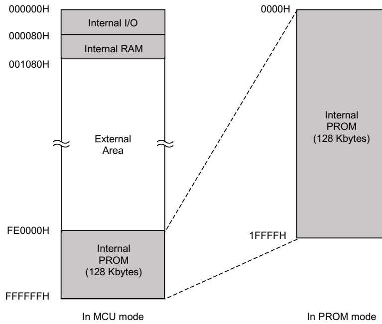
Figure 3.2.1 Memory map
