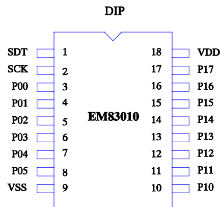
Fig. 1 Pin assignment
