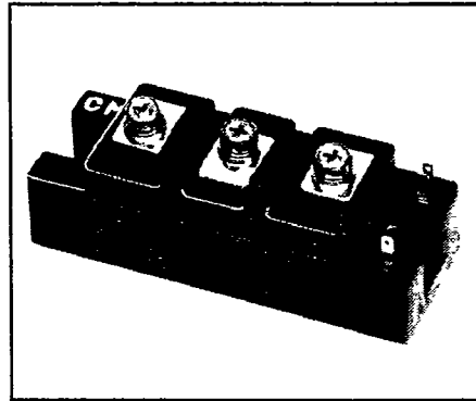
ID226075 Dual IGBTMOD™ Power Module 75 Amperes/600 Volts
