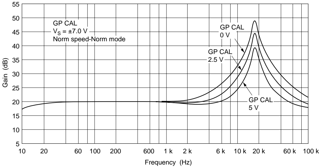
Equalizer Amp. Gain vs. Frequency (4)
