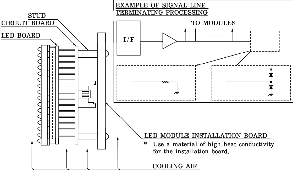
COOLING EXAMPLE
