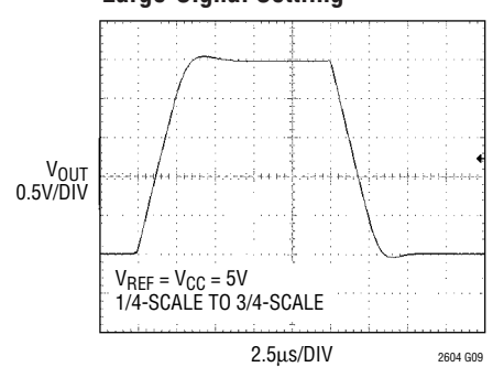
Large-Signal Settling
