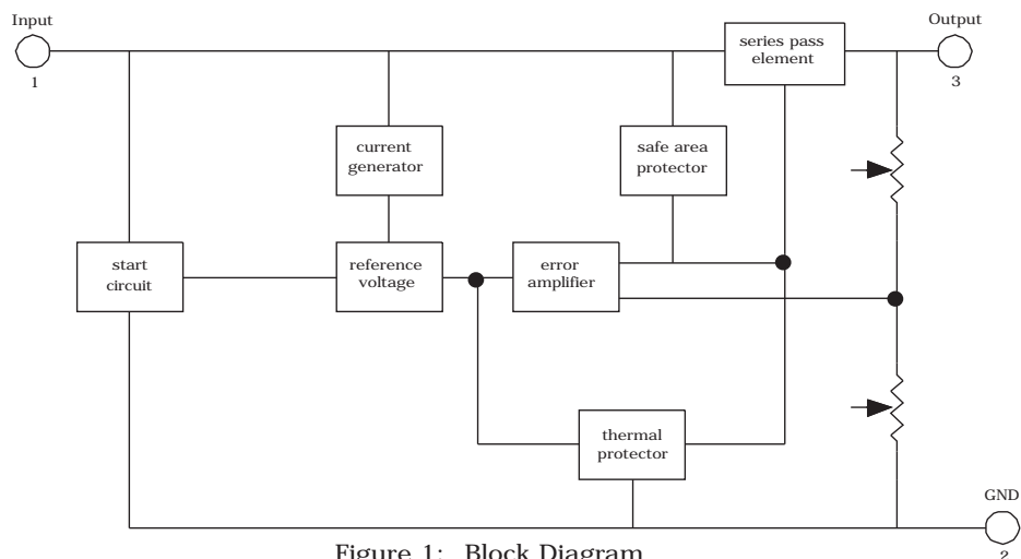
Figure 1: Block Diagram
