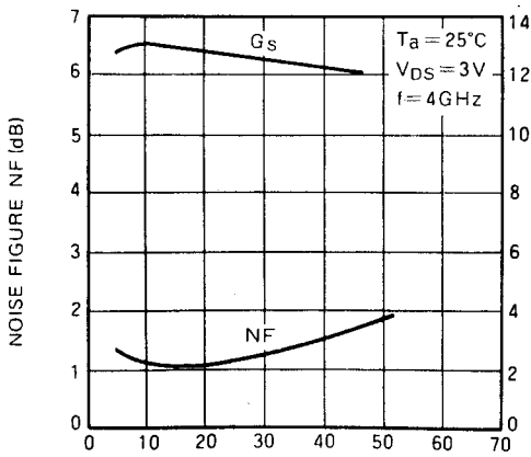
DRAIN CURRENT I_D (mA)
