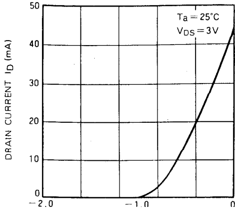
GATE TO SOURCE VOLTAGE V_{GS} (V)
