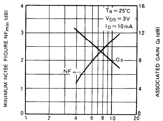
NF_{min} & G_s vs. f
