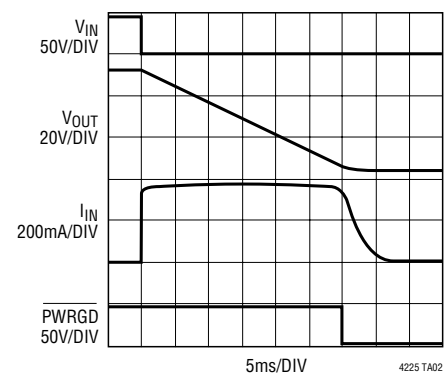
LTC4257 Charging 300 \mu F Load Capacitor
