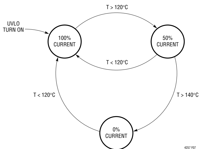
Figure 7. Smart Thermal Protection State Diagram
