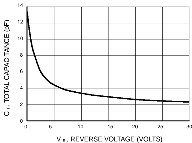
Figure 4. Total Capacitance
