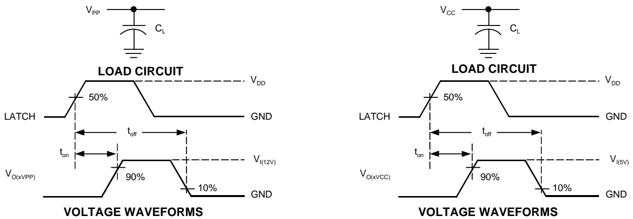
Figure 1. Test Circuits and Voltage Waveforms
