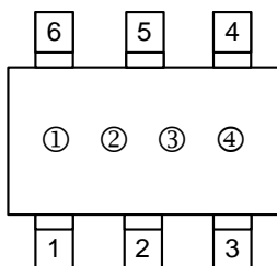
SOT-26 (TOP-VIEW)
