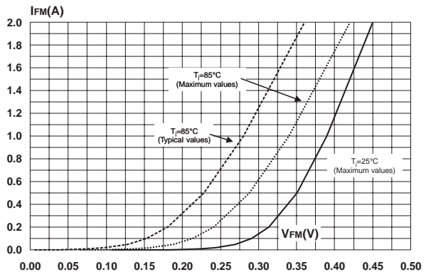
Fig. 10: Forward voltage drop versus forward current.
