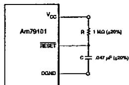
Figure 15a. Automatic Reset
