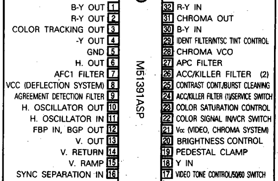
Outline 32P4B
