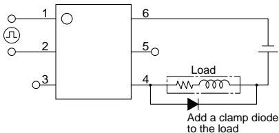
Non-latch type
