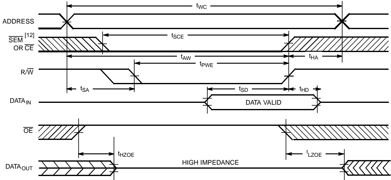
Write Cycle No. 2: R/\overline{W} Three-States Data I/Os (Either Port) [18, 20]
