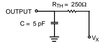
(c) Three-State Delay (Load 1)
