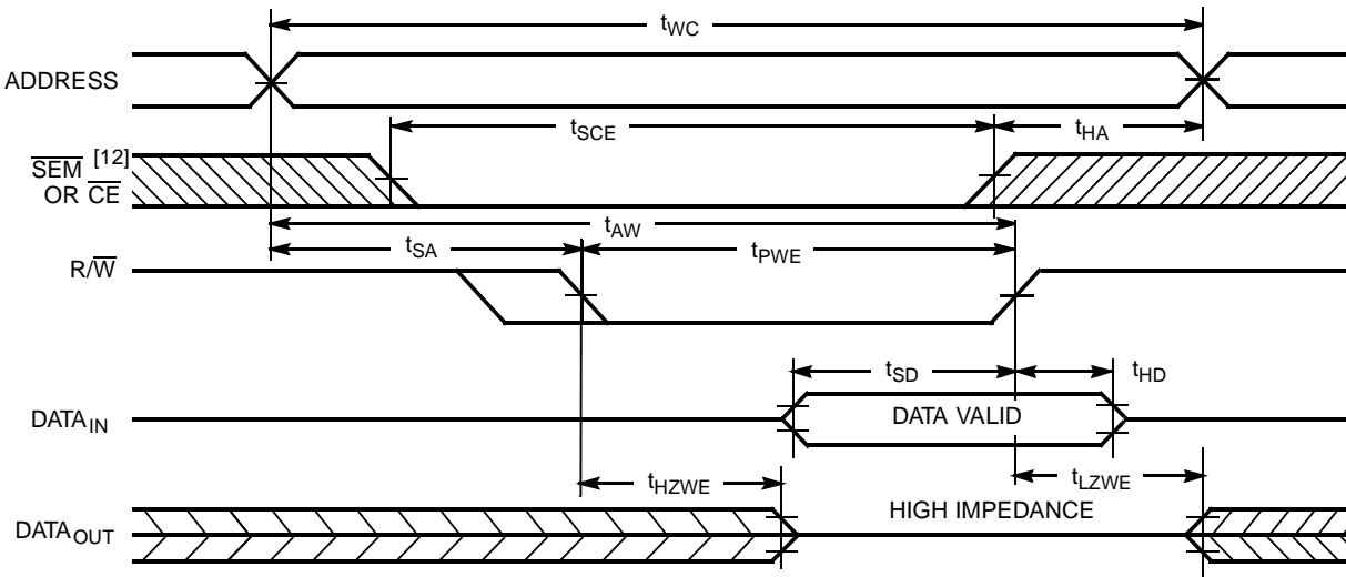
Write Cycle No. 2: R/\overline{W} Three-States Data I/Os (Either Port) [18, 20]
