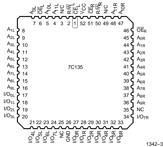
PLCC Top View
