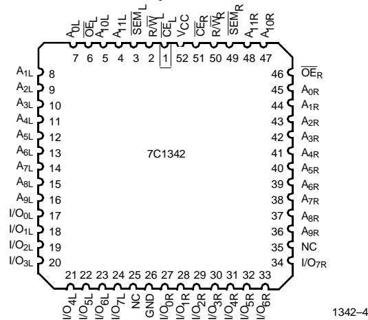
PLCC Top View
