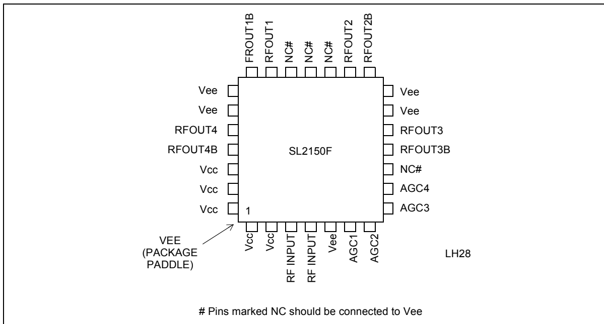
Figure 2 - Pin Allocation
