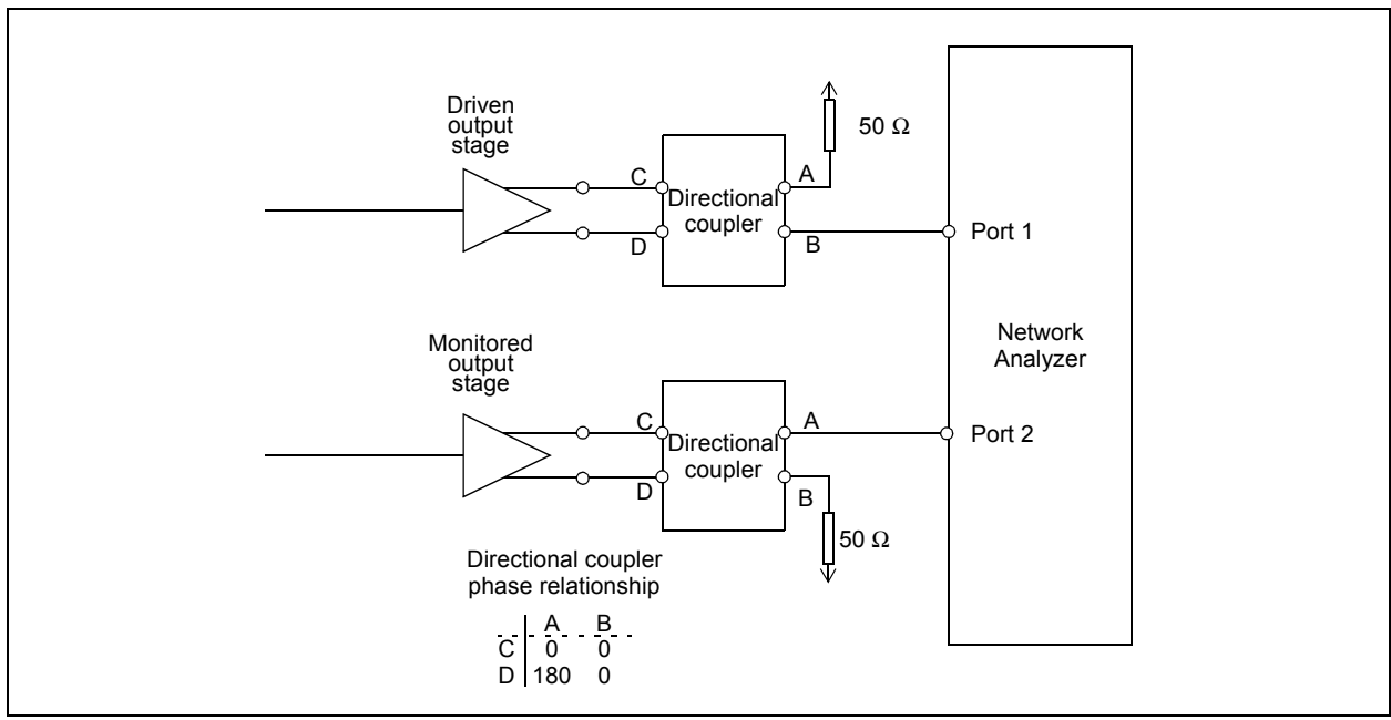
Figure 10 - Test Condition for Output Crosstalk
