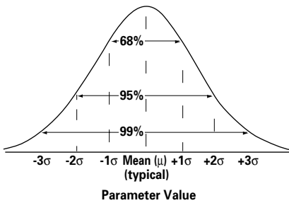
Figure 14. Normal Distribution.
