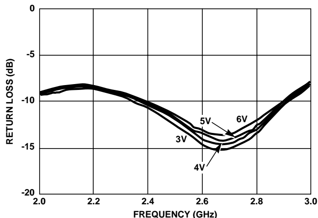
FIGURE 3. OUTPUT MATCH
