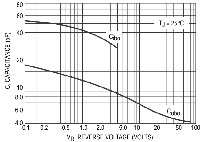
Figure 3. Capacitance
