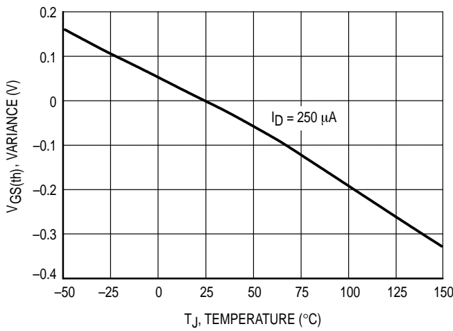
Figure 9. Threshold Voltage
