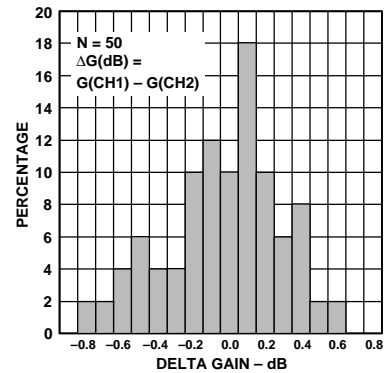
Figure 9. Gain Match, VGN_1 = VGN_2 = 2.50\text{ V}
