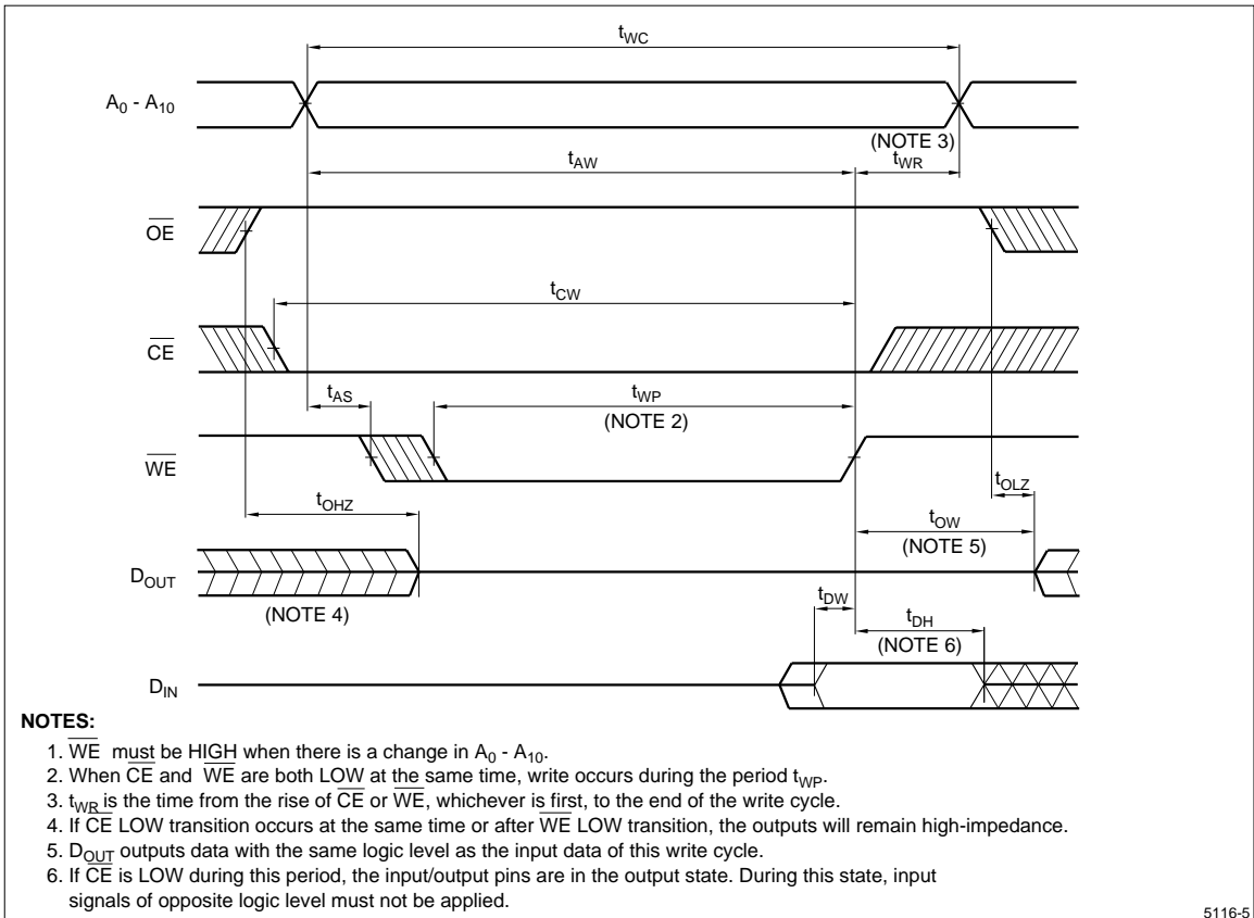
Figure 6. Write Cycle 2
