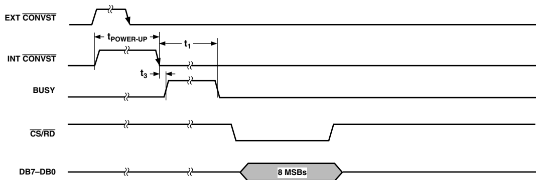
Figure 14. Mode 2 Operation
